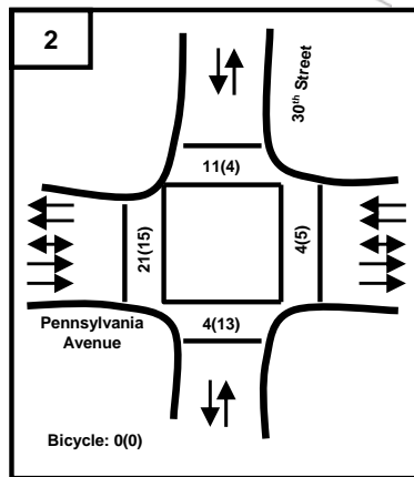
FIGURE 16: 2007 EXISTING AM(PM) PEAK HOUR PEDESTRAIN VOLUMES
